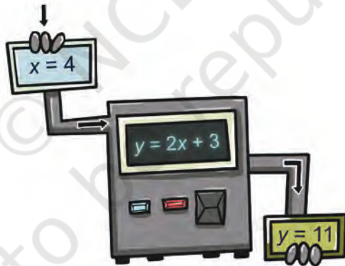
Fig. 2.3: A linear expression as an input-output process
