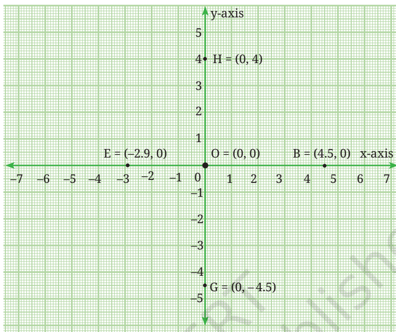
Fig. 1.2: Structure of the coordinate plane
